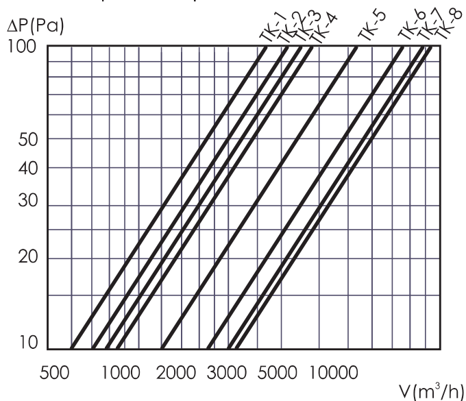
Pressure drop on a damper
